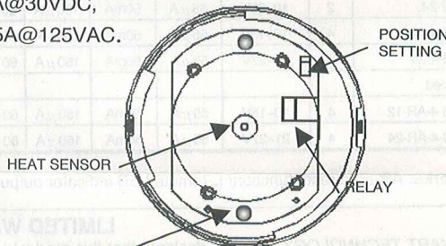
Fig. 3 Schematic of detector structure When front cover is open.
